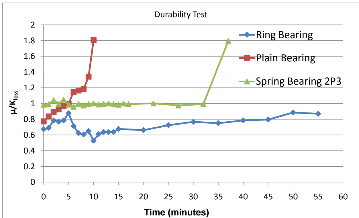
Figure: 9 Durability Test for three Bearing Styles
